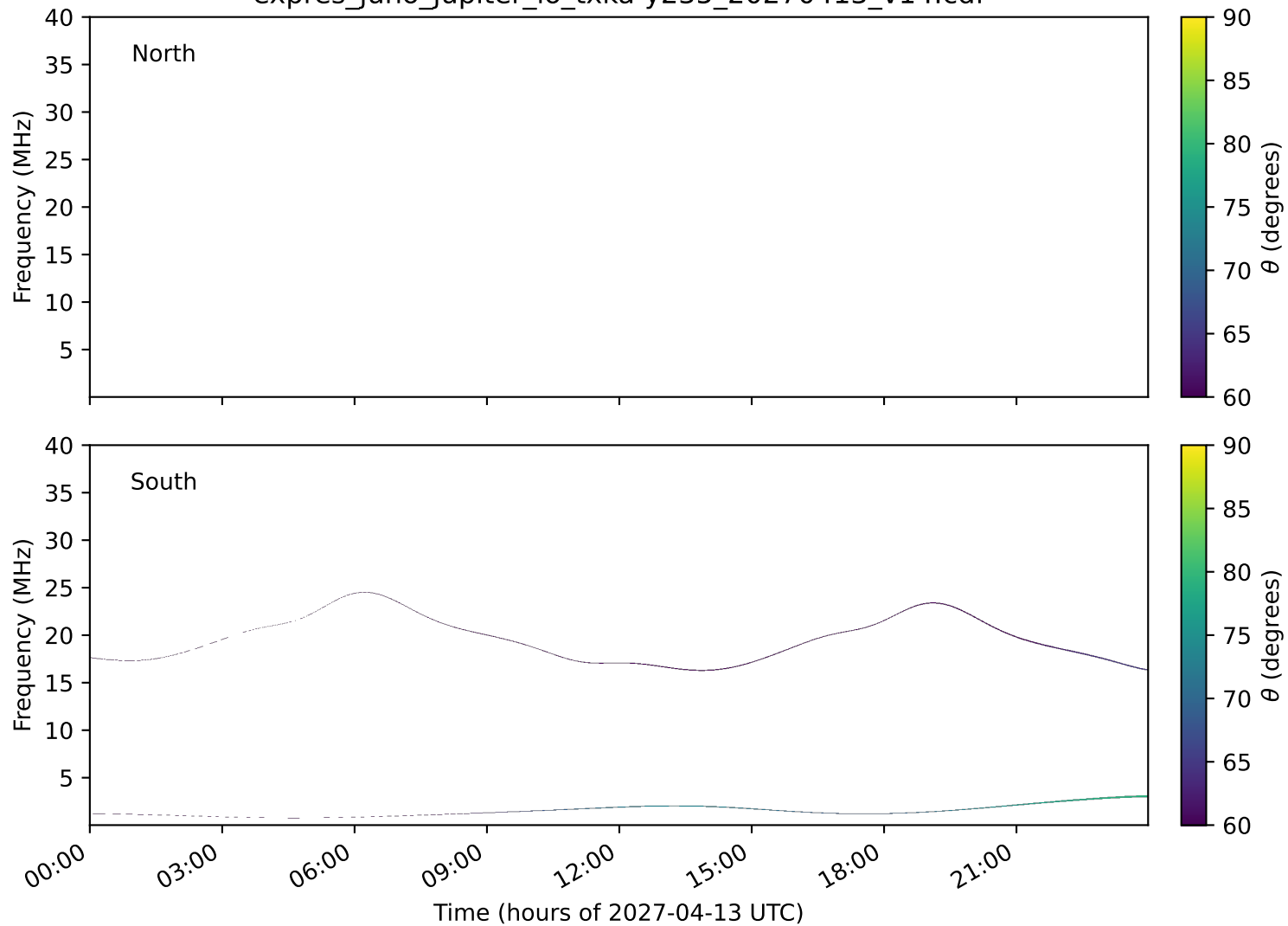
expres_juno_jupiter_io_txka-y235_20270413_v14.cdf
