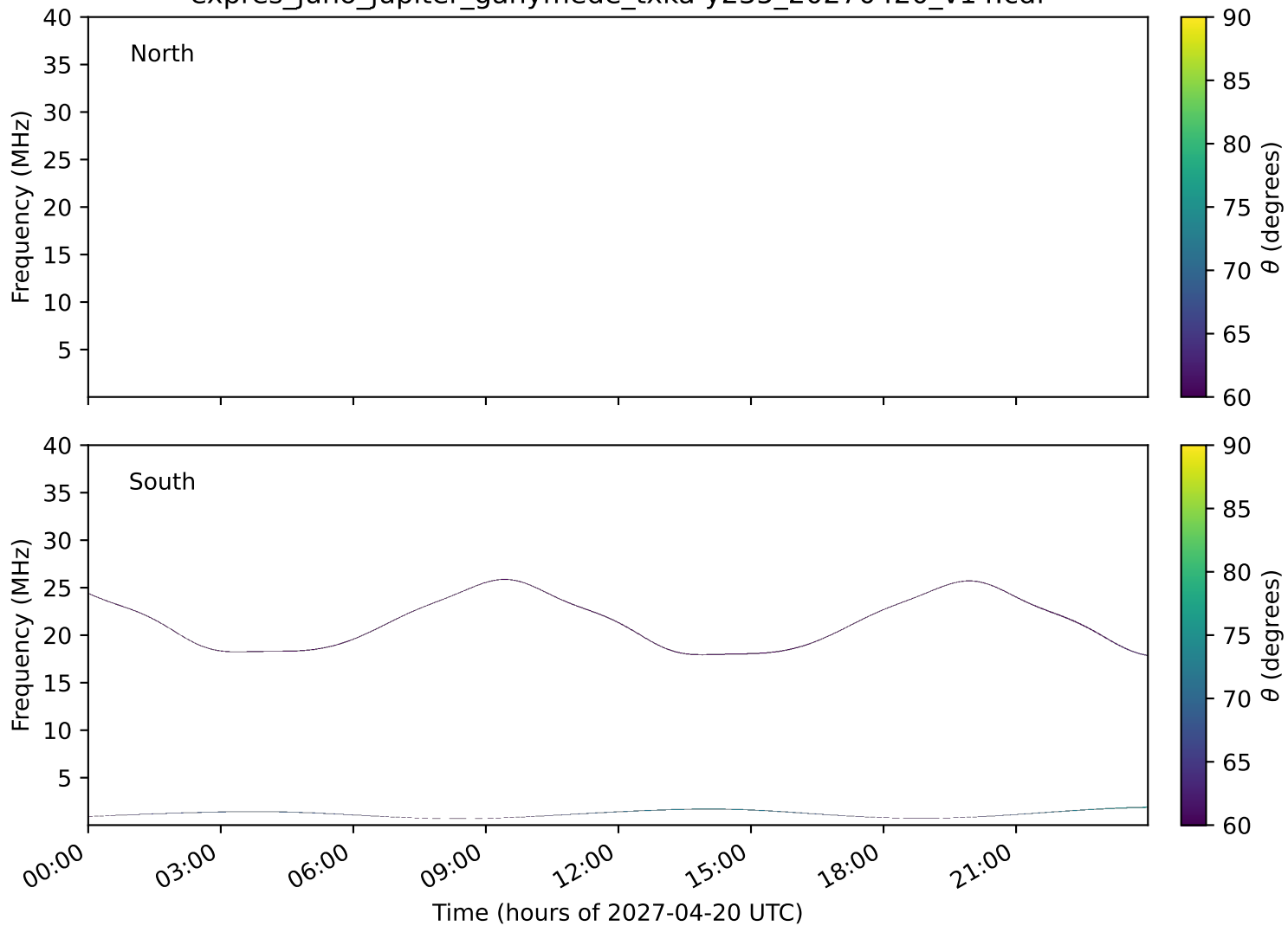
expres_juno_jupiter_ganymede_txka-y235_20270420_v14.cdf
