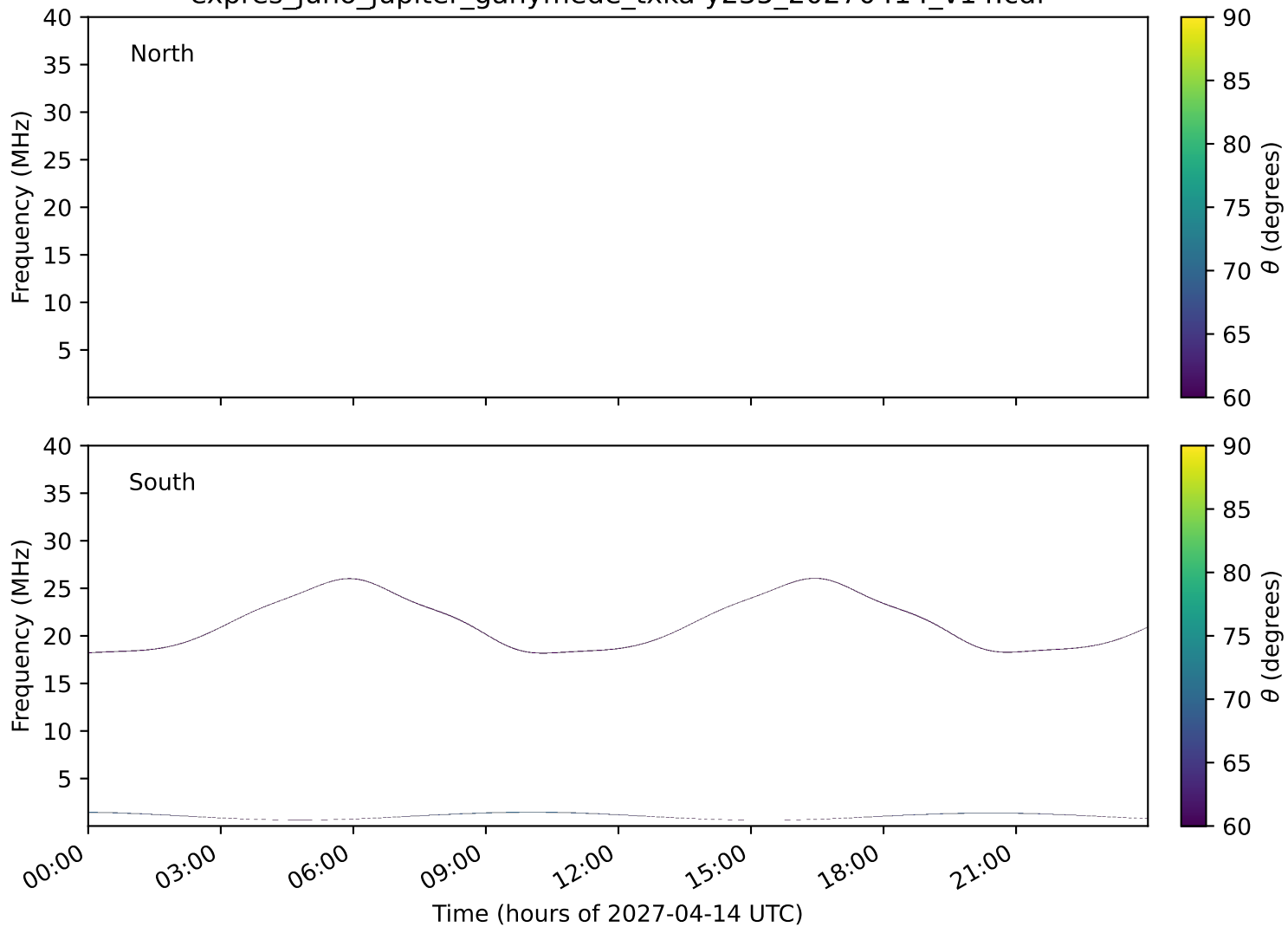
expres_juno_jupiter_ganymede_txka-y235_20270414_v14.cdf
