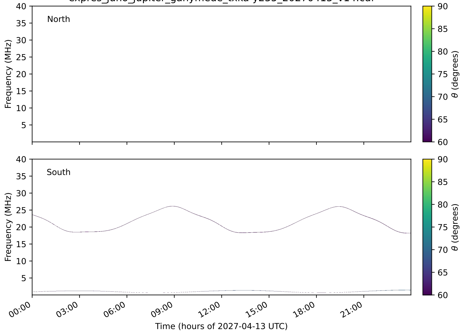
expres_juno_jupiter_ganymede_txka-y235_20270413_v14.cdf
