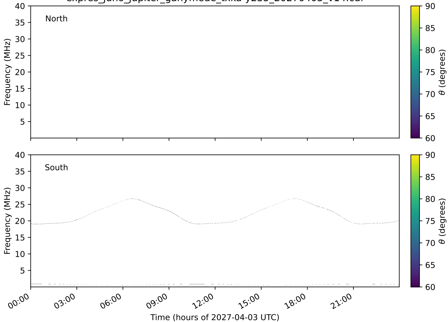
expres_juno_jupiter_ganymede_txka-y235_20270403_v14.cdf
