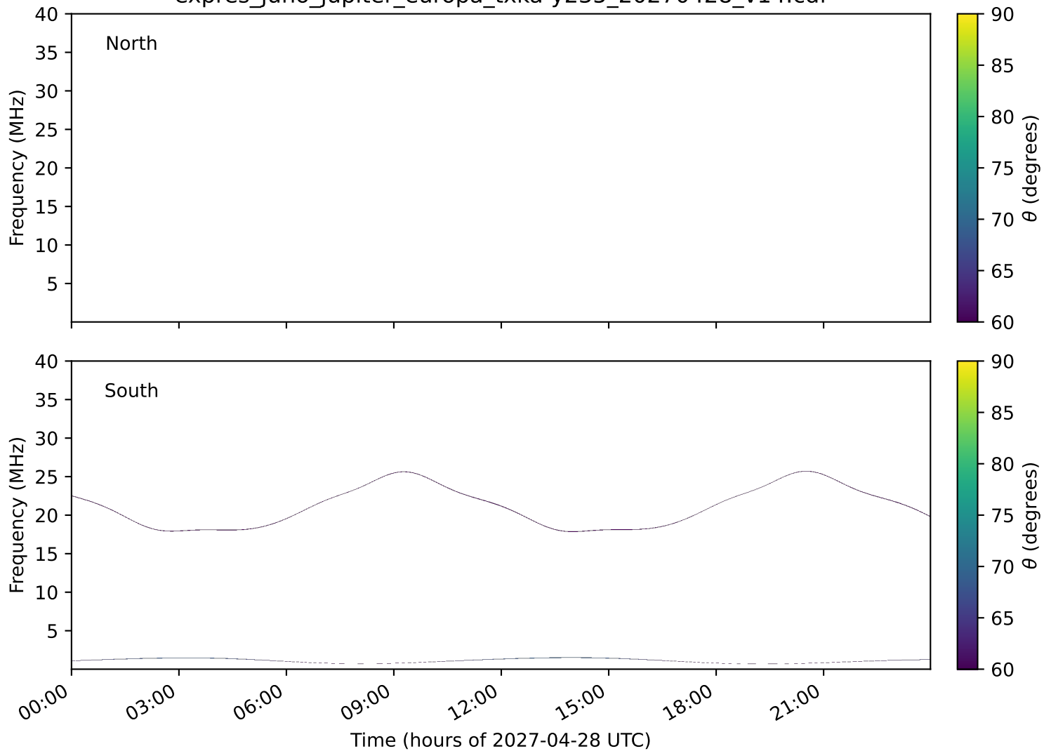
expres_juno_jupiter_europa_txka-y235_20270428_v14.cdf
