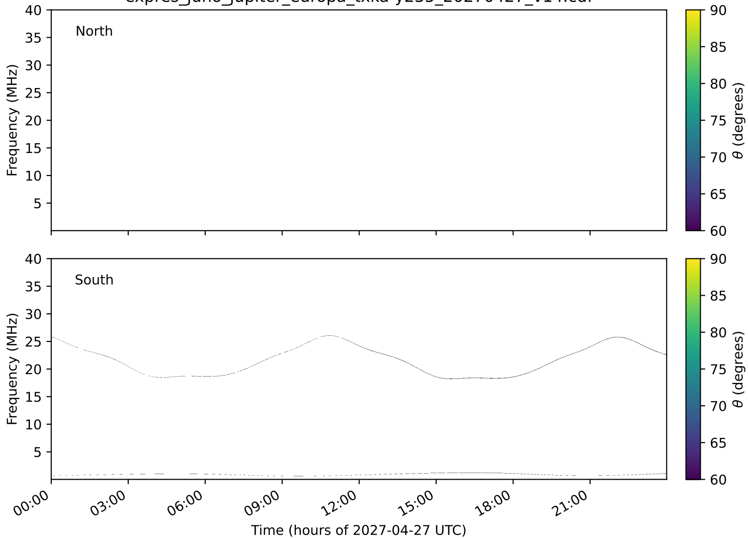
expres_juno_jupiter_europa_txka-y235_20270427_v14.cdf
