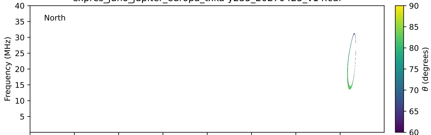
expres_juno_jupiter_europa_txka-y235_20270425_v14.cdf
