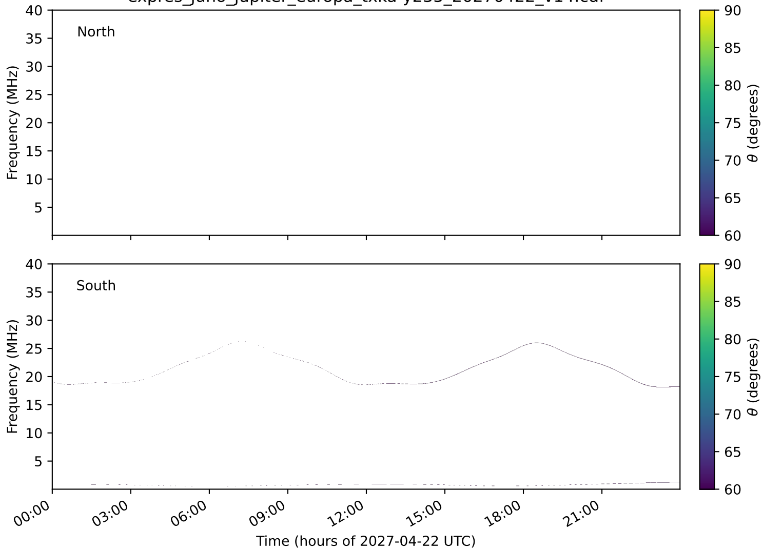
expres_juno_jupiter_europa_txka-y235_20270422_v14.cdf
