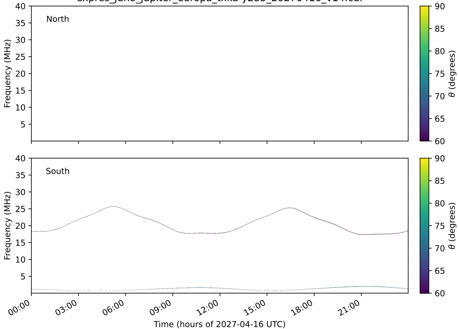
expres_juno_jupiter_europa_txka-y235_20270416_v14.cdf
