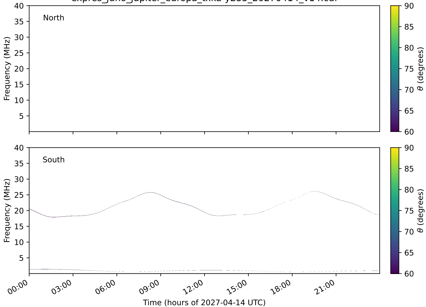
expres_juno_jupiter_europa_txka-y235_20270414_v14.cdf
