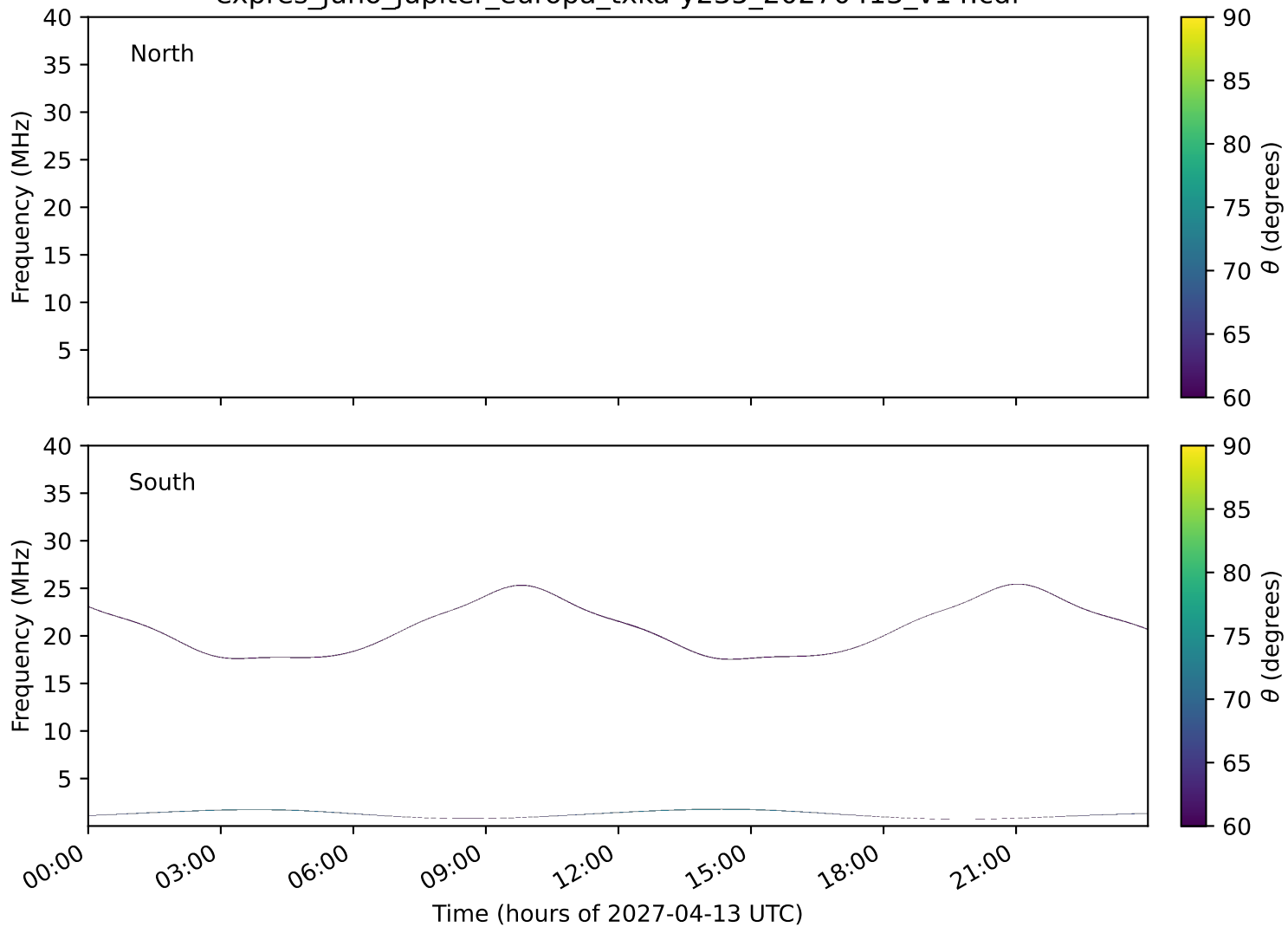
expres_juno_jupiter_europa_txka-y235_20270413_v14.cdf
