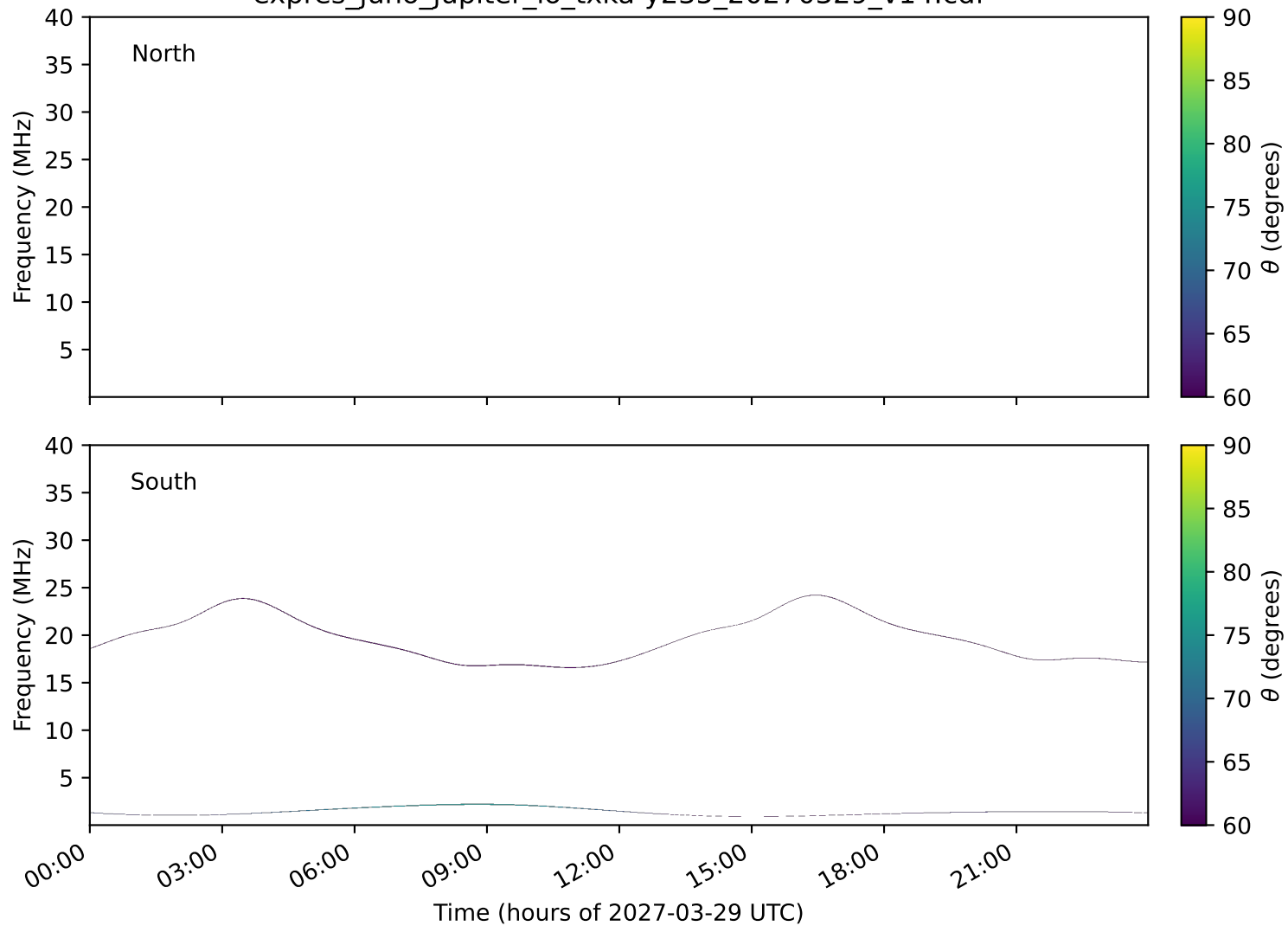
expres_juno_jupiter_io_txka-y235_20270329_v14.cdf
