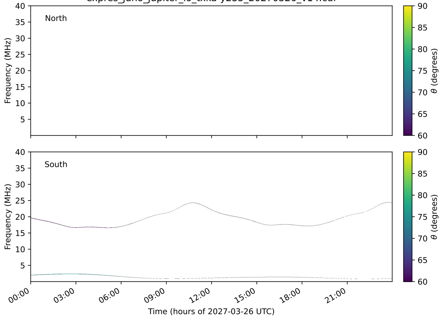
expres_juno_jupiter_io_txka-y235_20270326_v14.cdf
