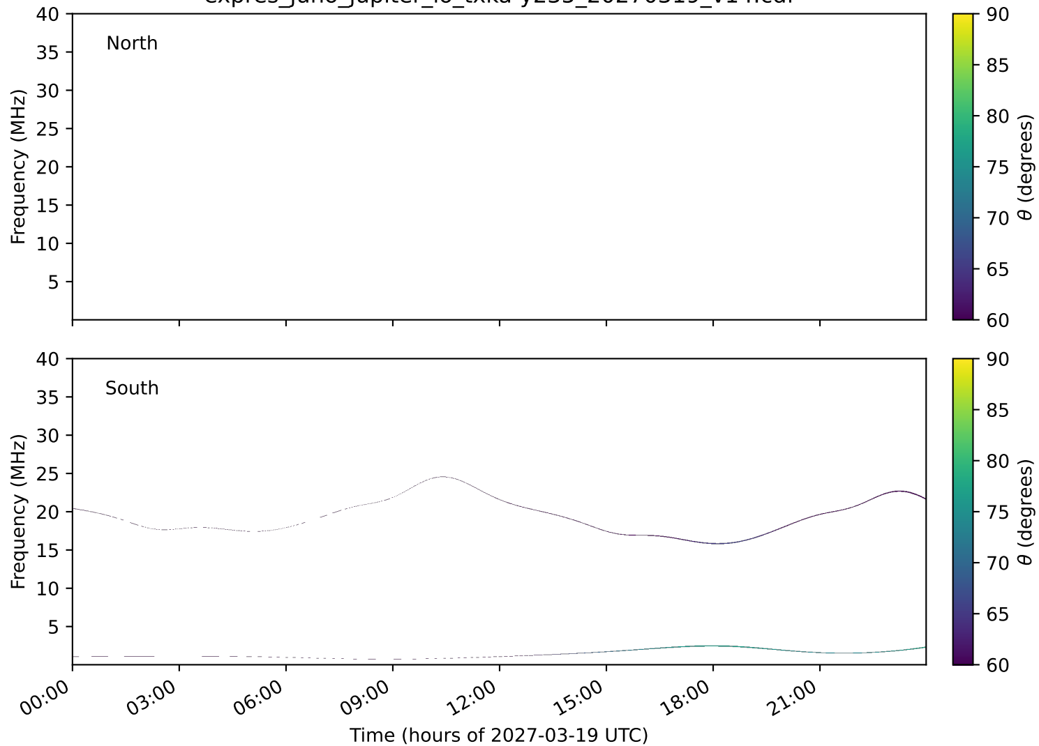
expres_juno_jupiter_io_txka-y235_20270319_v14.cdf
