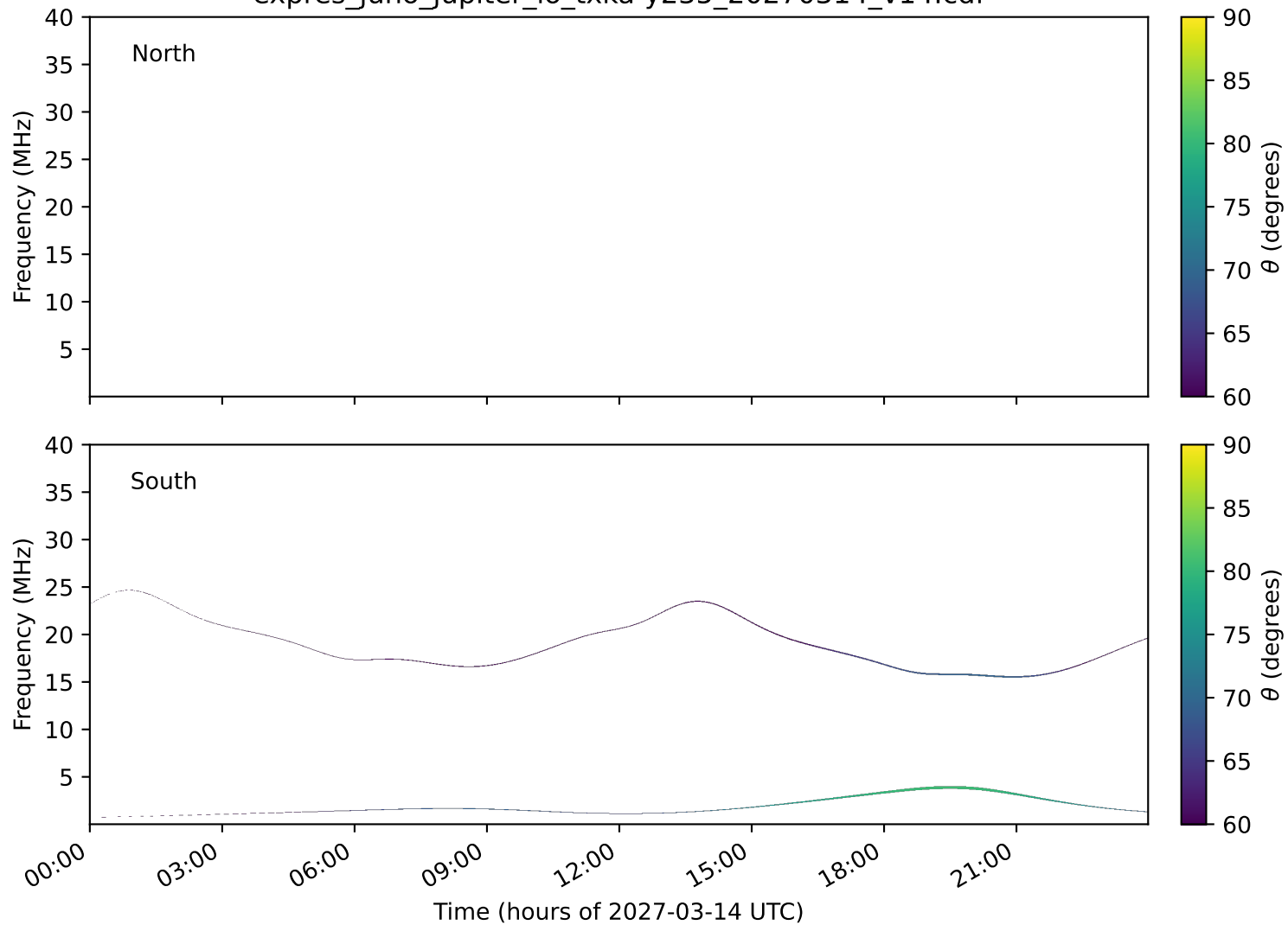
expres_juno_jupiter_io_txka-y235_20270314_v14.cdf
