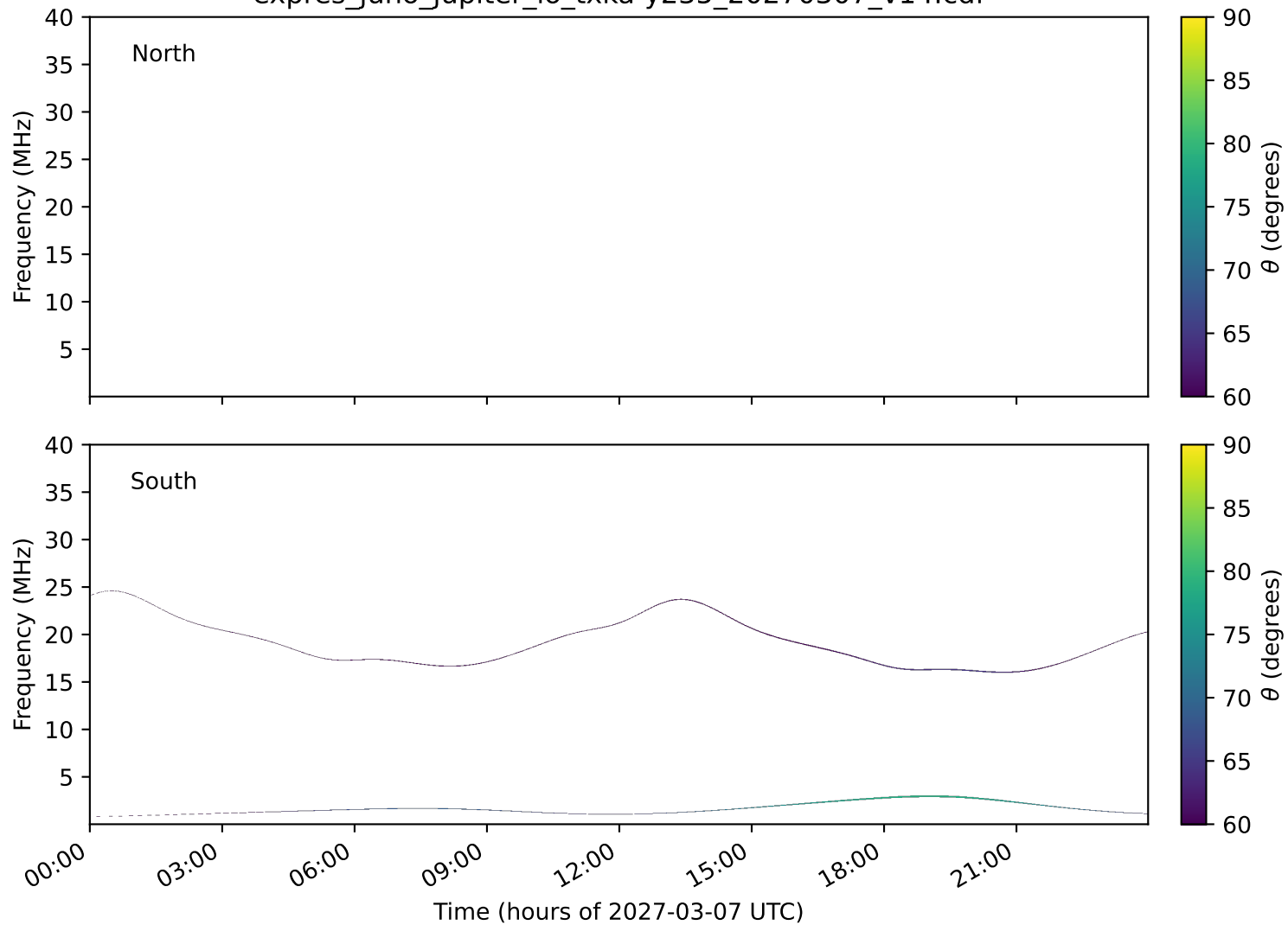
expres_juno_jupiter_io_txka-y235_20270307_v14.cdf
