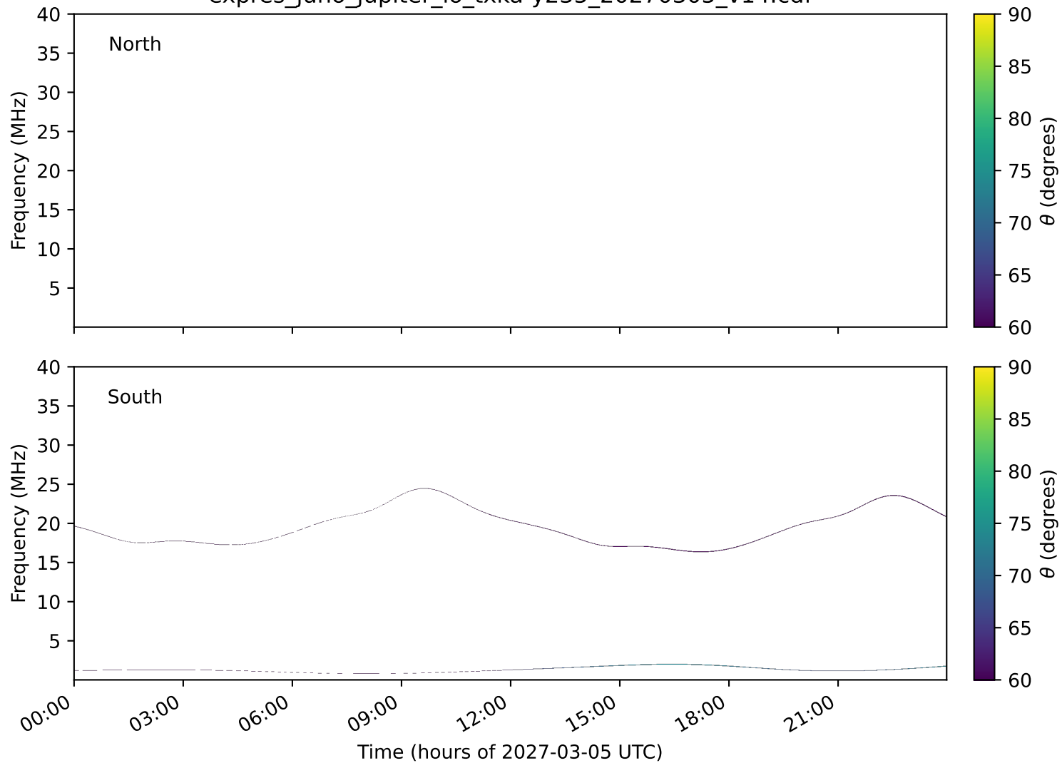
expres_juno_jupiter_io_txka-y235_20270305_v14.cdf
