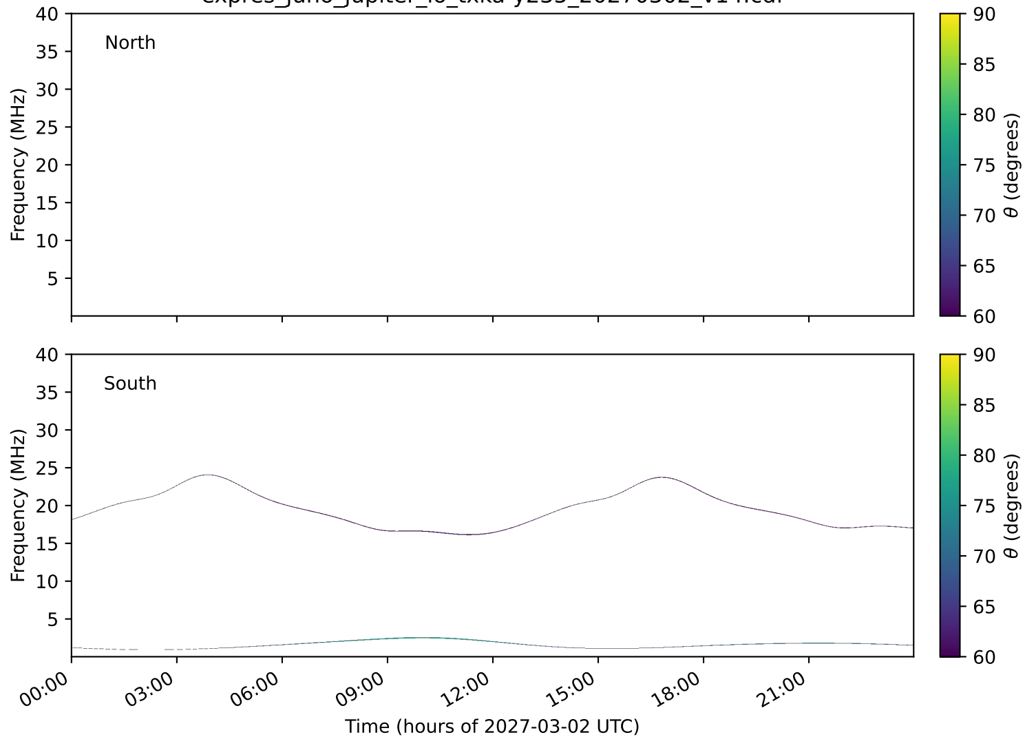
expres_juno_jupiter_io_txka-y235_20270302_v14.cdf
