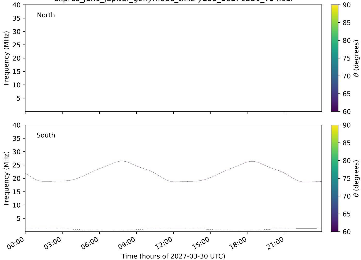
expres_juno_jupiter_ganymede_txka-y235_20270330_v14.cdf
