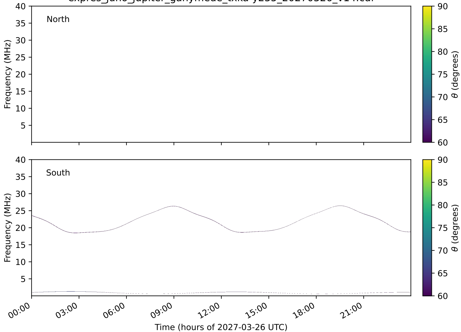
expres_juno_jupiter_ganymede_txka-y235_20270326_v14.cdf
