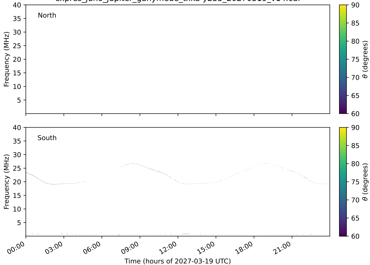
expres_juno_jupiter_ganymede_txka-y235_20270319_v14.cdf
