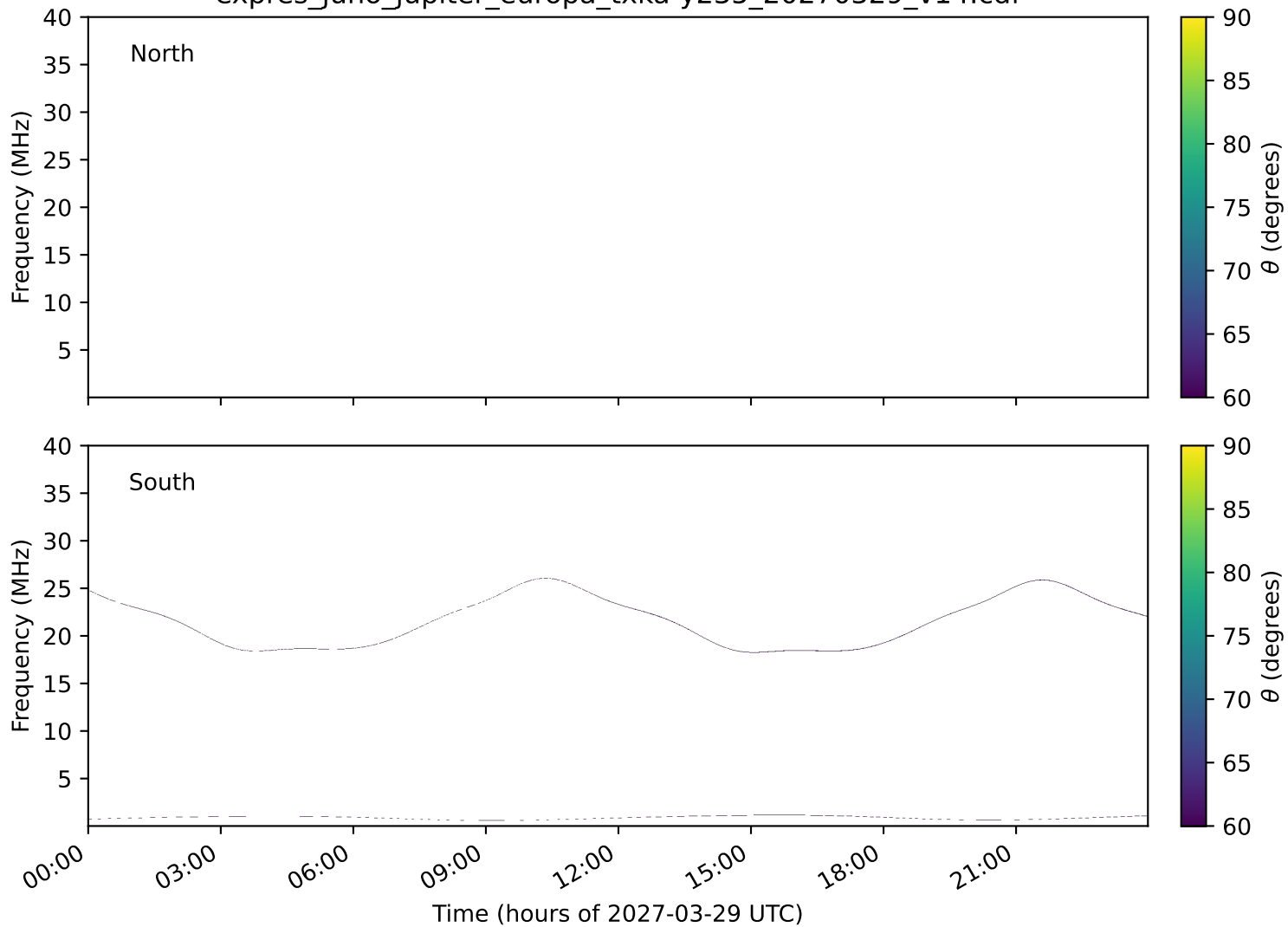
expres_juno_jupiter_europa_txka-y235_20270329_v14.cdf
