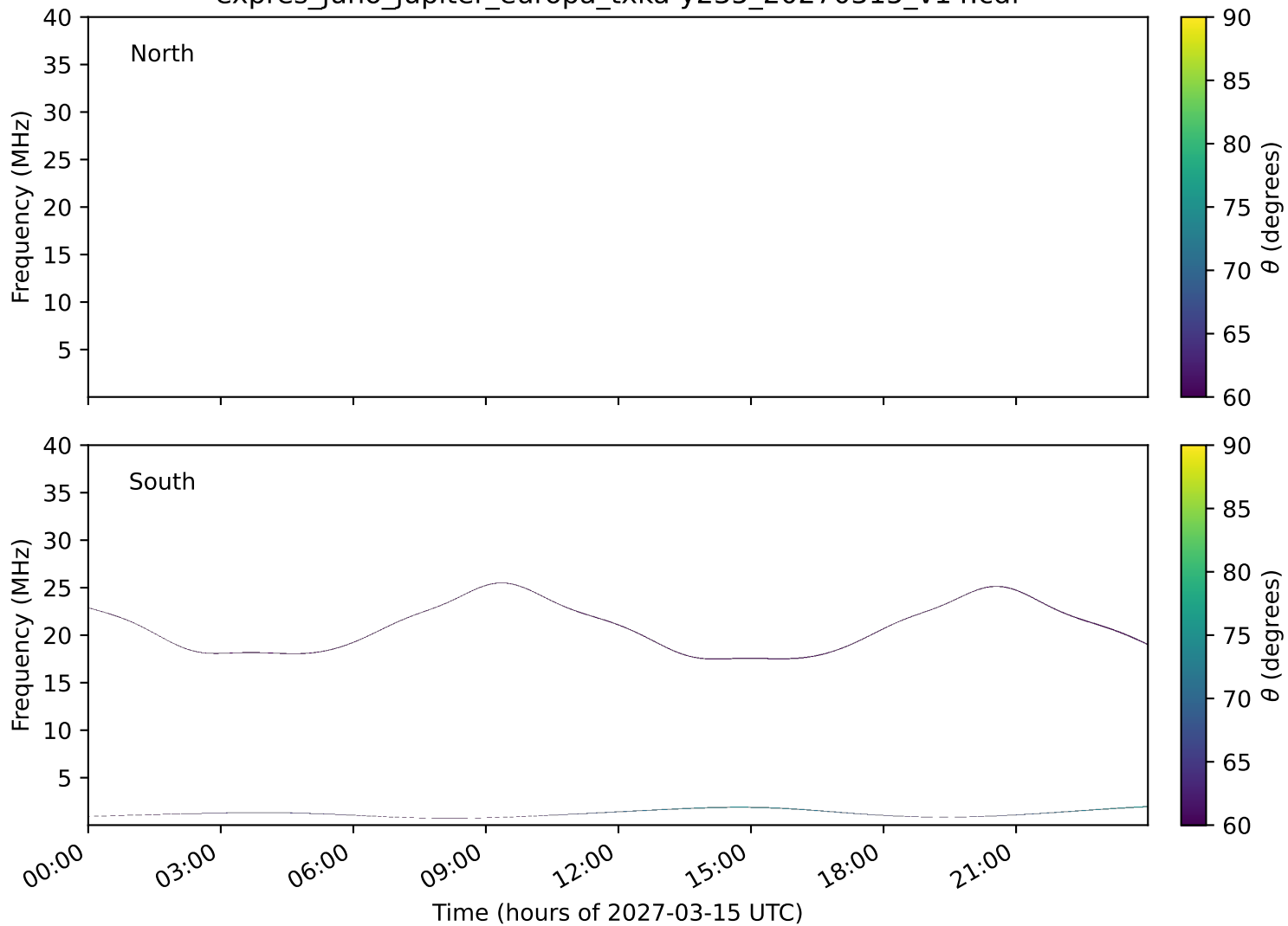
expres_juno_jupiter_europa_txka-y235_20270315_v14.cdf
