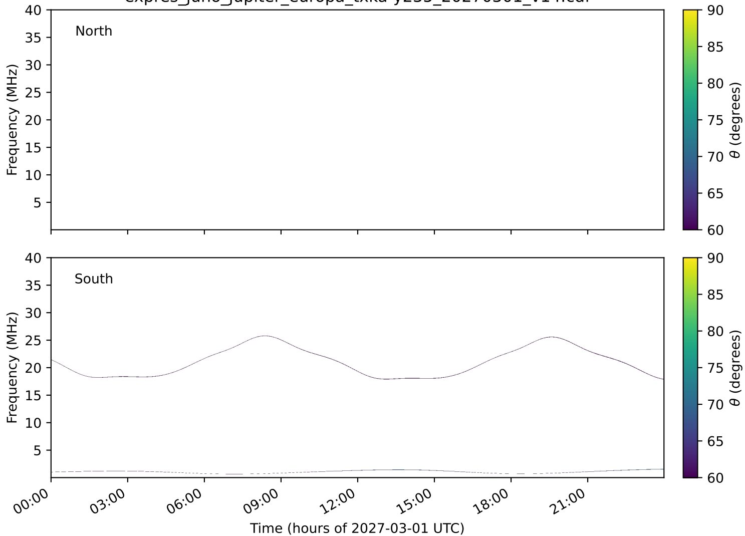
expres_juno_jupiter_europa_txka-y235_20270301_v14.cdf
