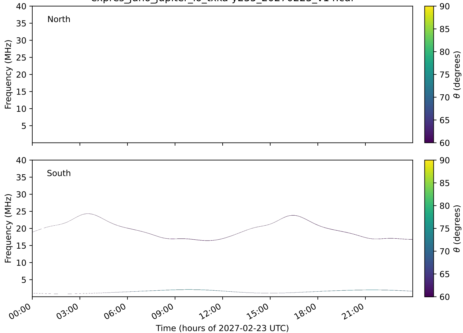
expres_juno_jupiter_io_txka-y235_20270223_v14.cdf
