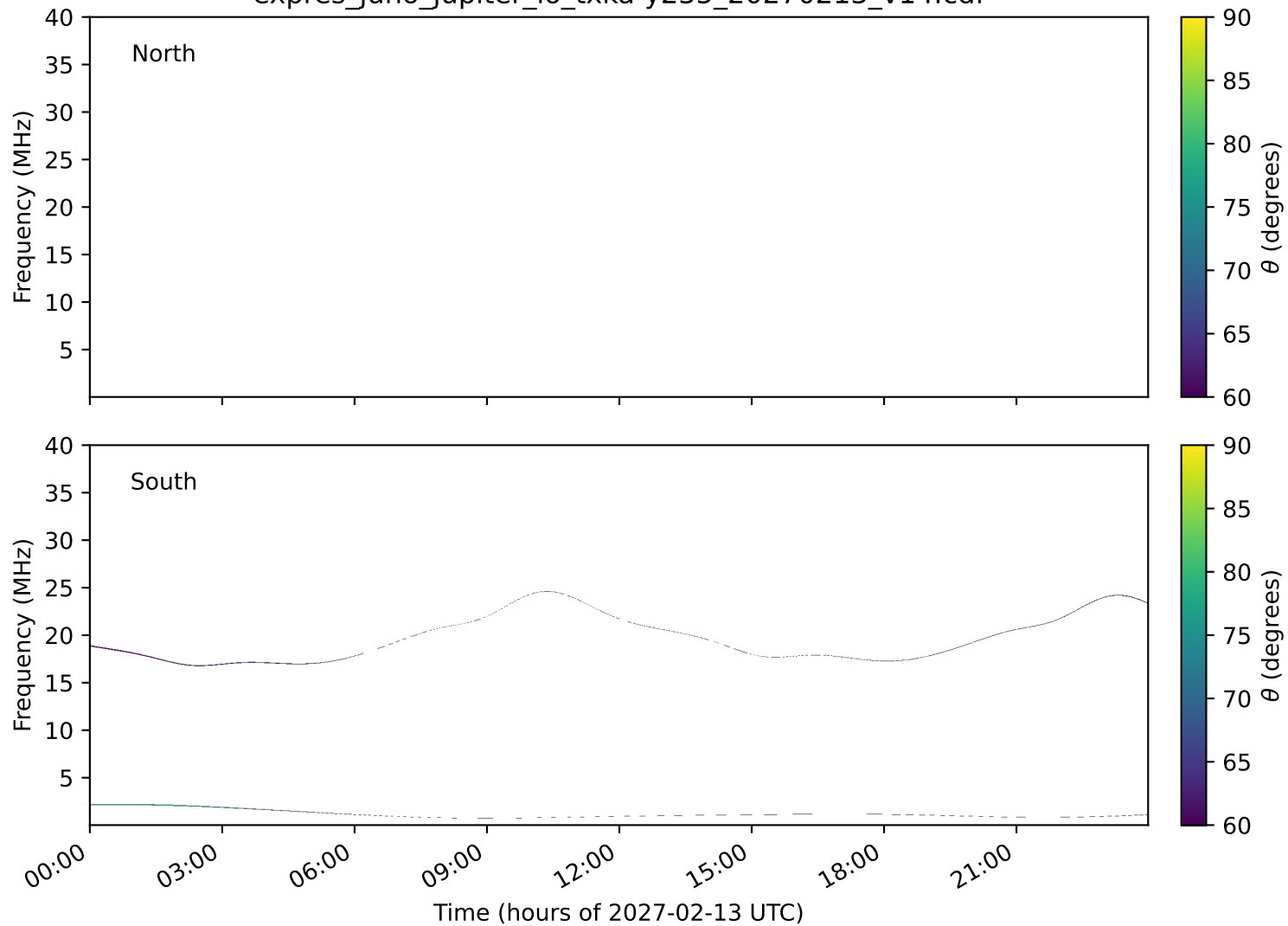
expres_juno_jupiter_io_txka-y235_20270213_v14.cdf
