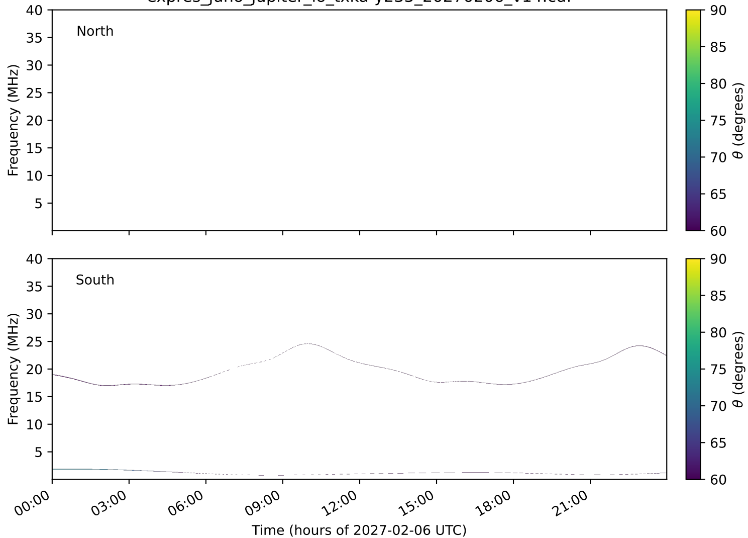
expres_juno_jupiter_io_txka-y235_20270206_v14.cdf
