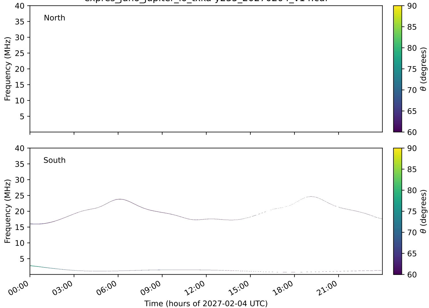
expres_juno_jupiter_io_txka-y235_20270204_v14.cdf
