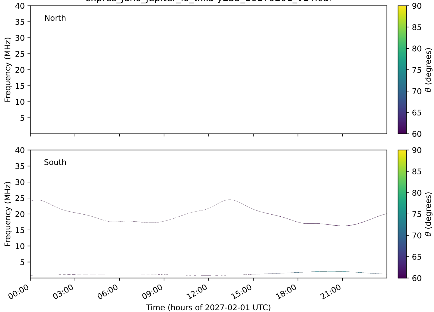
expres_juno_jupiter_io_txka-y235_20270201_v14.cdf
