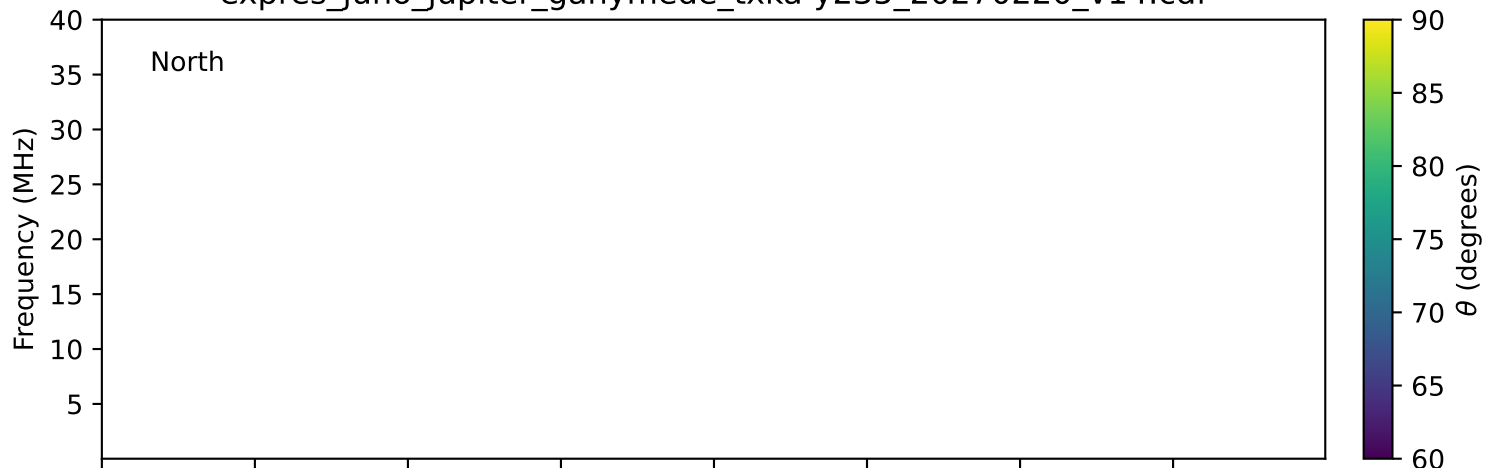
expres_juno_jupiter_ganymede_txka-y235_20270220_v14.cdf
