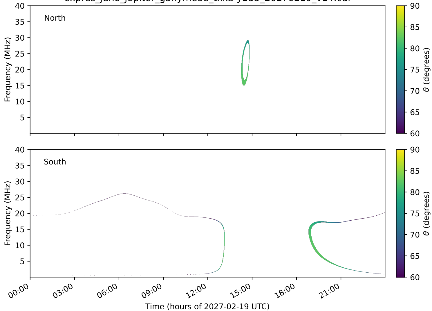
expres_juno_jupiter_ganymede_txka-y235_20270219_v14.cdf
