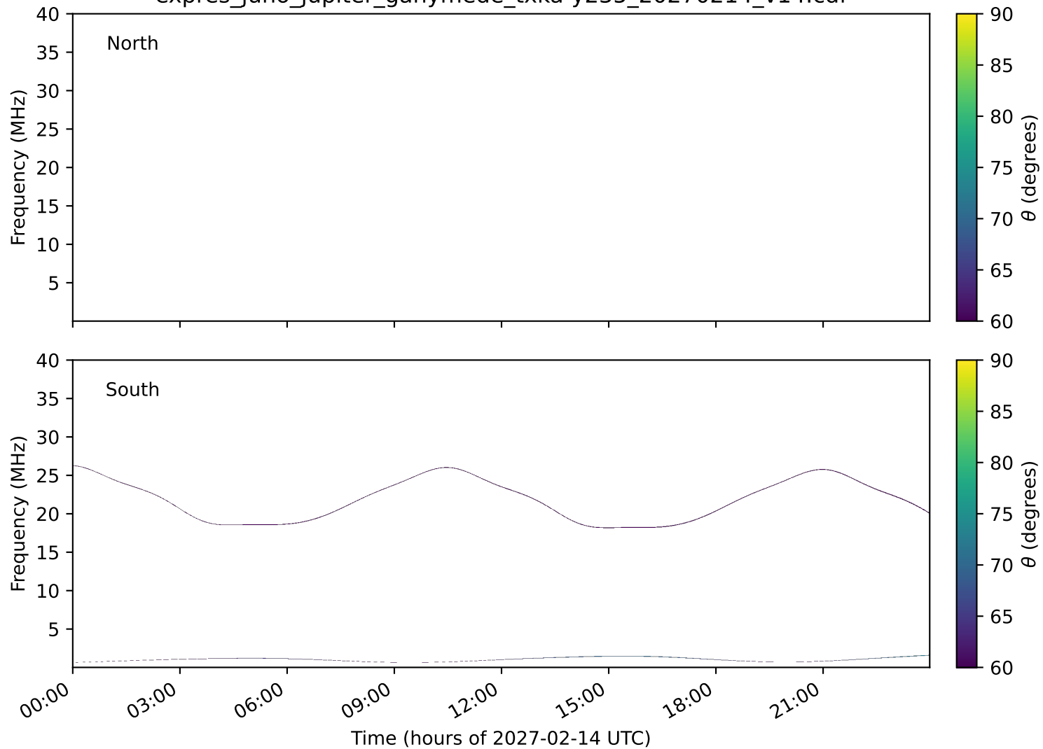
expres_juno_jupiter_ganymede_txka-y235_20270214_v14.cdf
