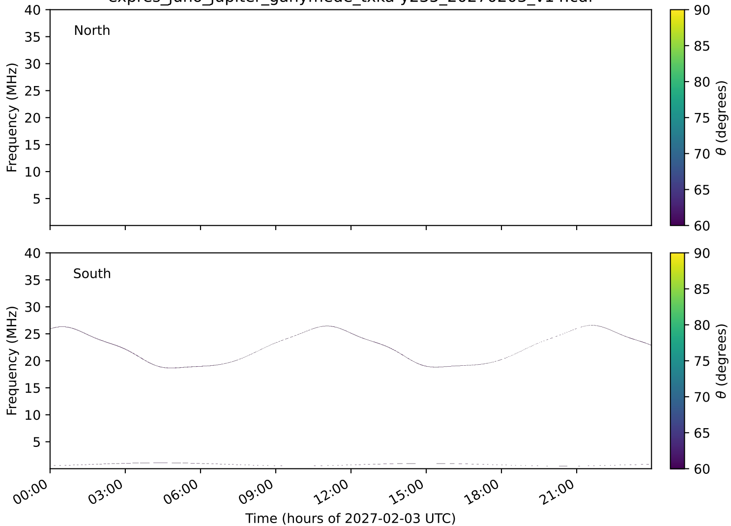
expres_juno_jupiter_ganymede_txka-y235_20270203_v14.cdf
