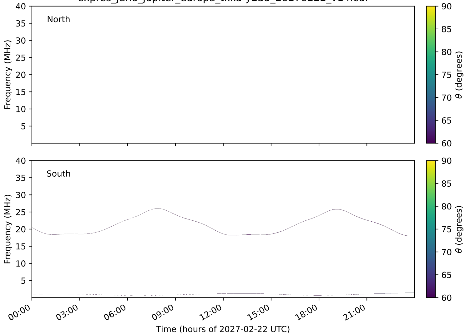
expres_juno_jupiter_europa_txka-y235_20270222_v14.cdf
