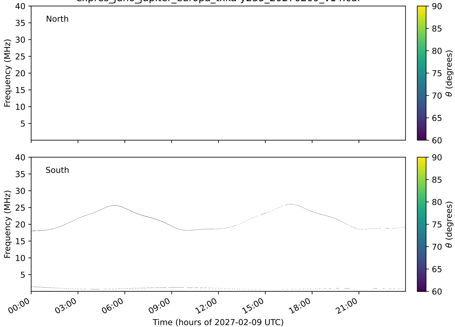
expres_juno_jupiter_europa_txka-y235_20270209_v14.cdf
