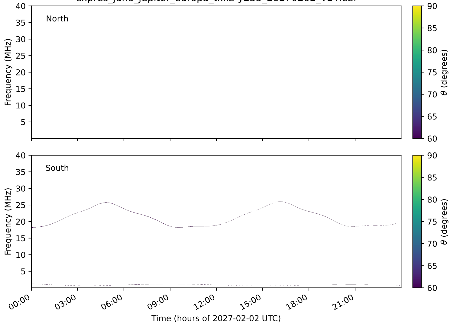
expres_juno_jupiter_europa_txka-y235_20270202_v14.cdf
