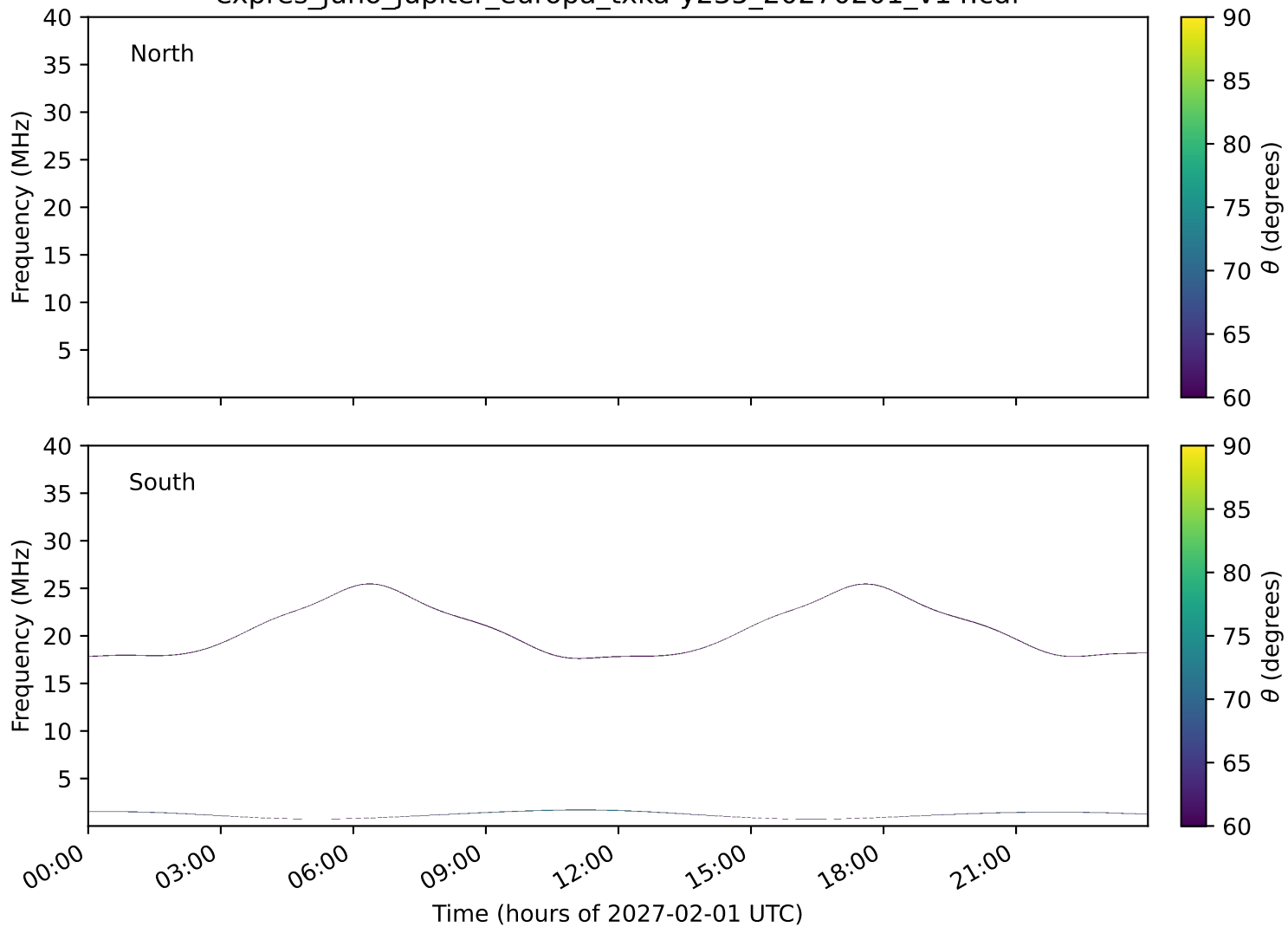
expres_juno_jupiter_europa_txka-y235_20270201_v14.cdf
