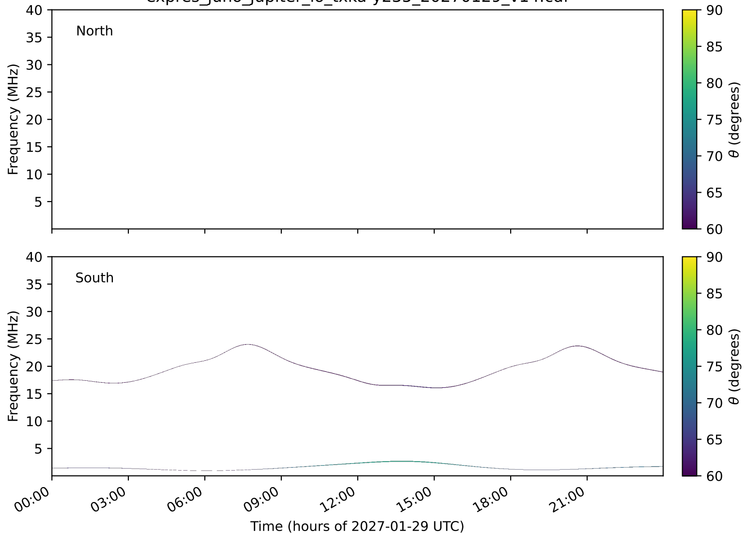
expres_juno_jupiter_io_txka-y235_20270129_v14.cdf
