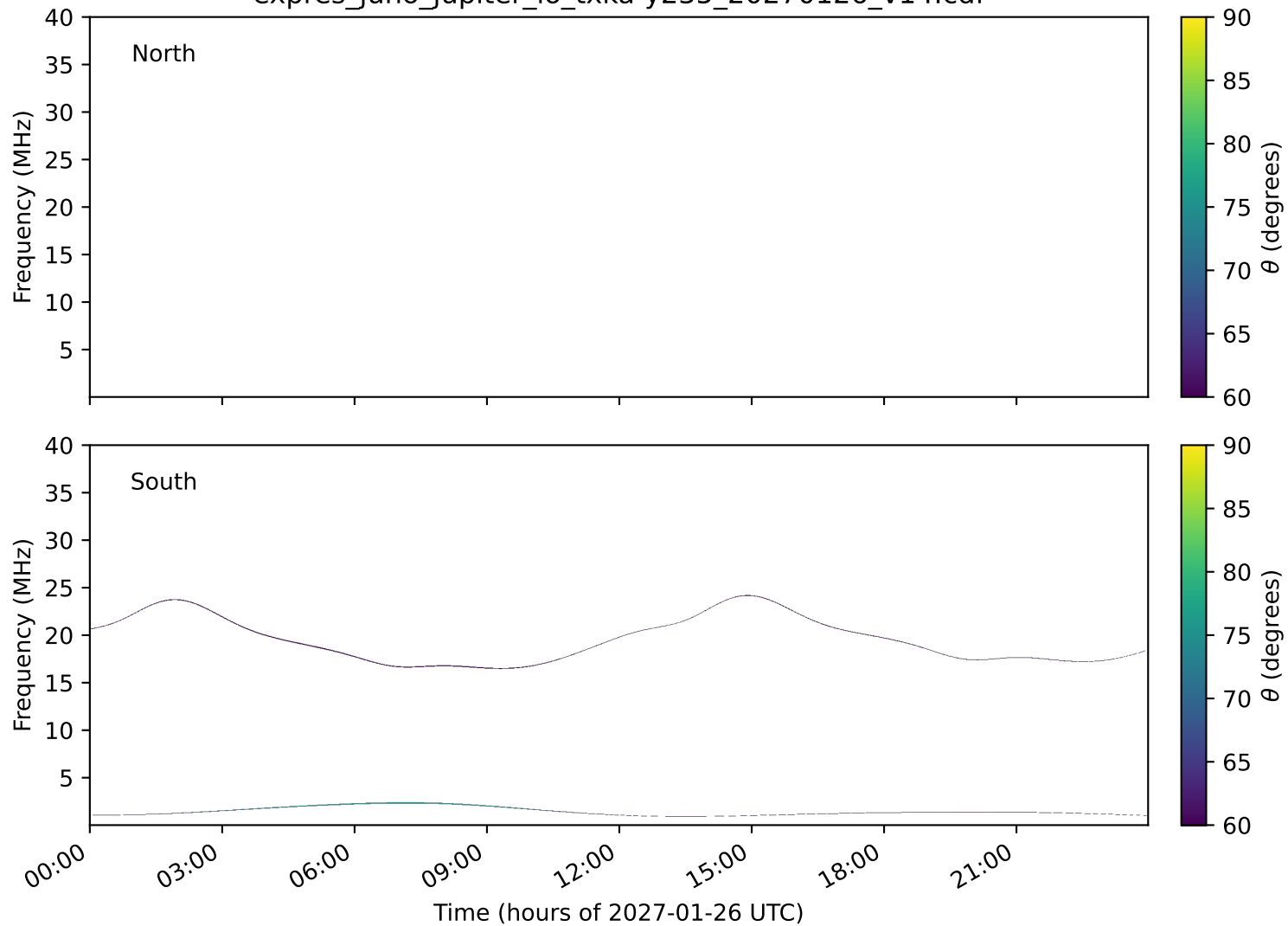
expres_juno_jupiter_io_txka-y235_20270126_v14.cdf
