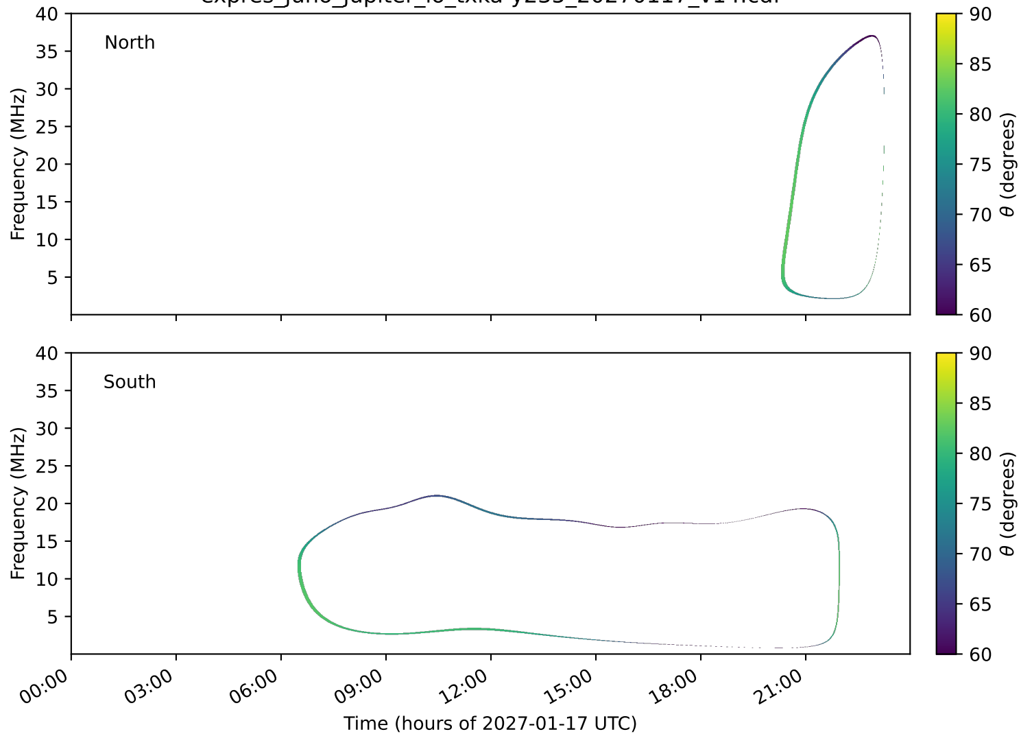
expres_juno_jupiter_io_txka-y235_20270117_v14.cdf
