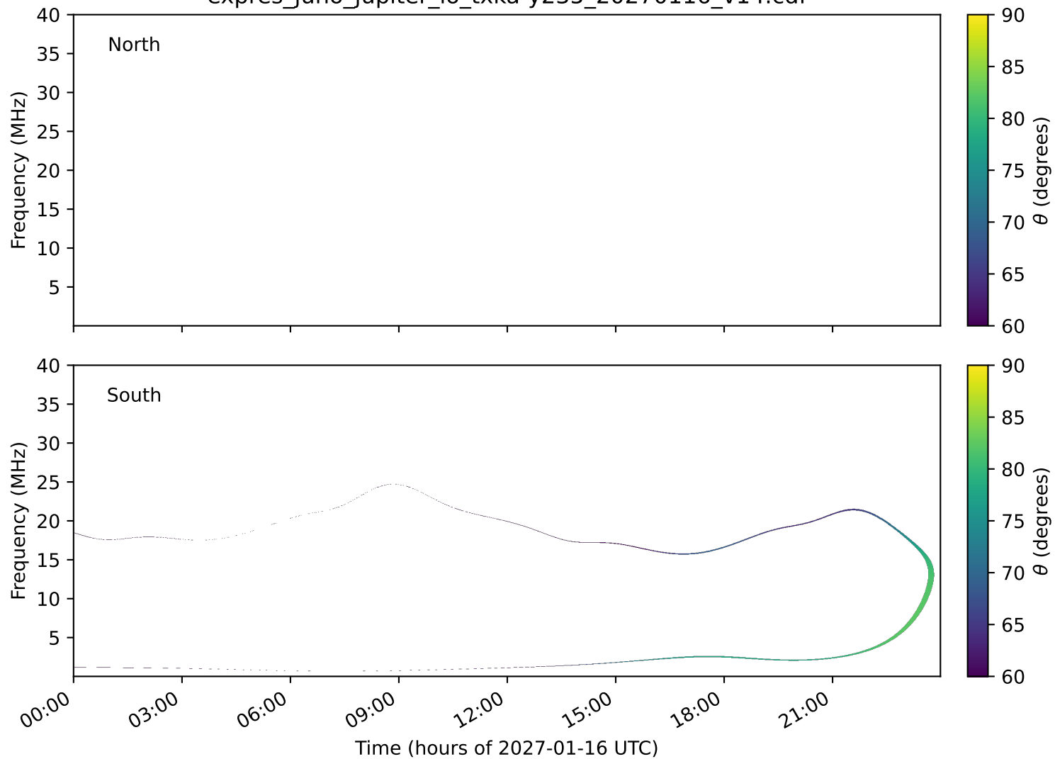
expres_juno_jupiter_io_txka-y235_20270116_v14.cdf
