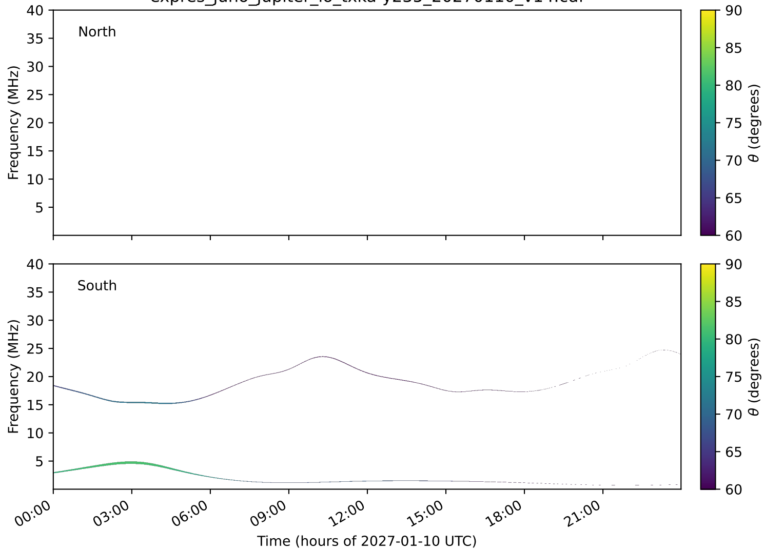
expres_juno_jupiter_io_txka-y235_20270110_v14.cdf
