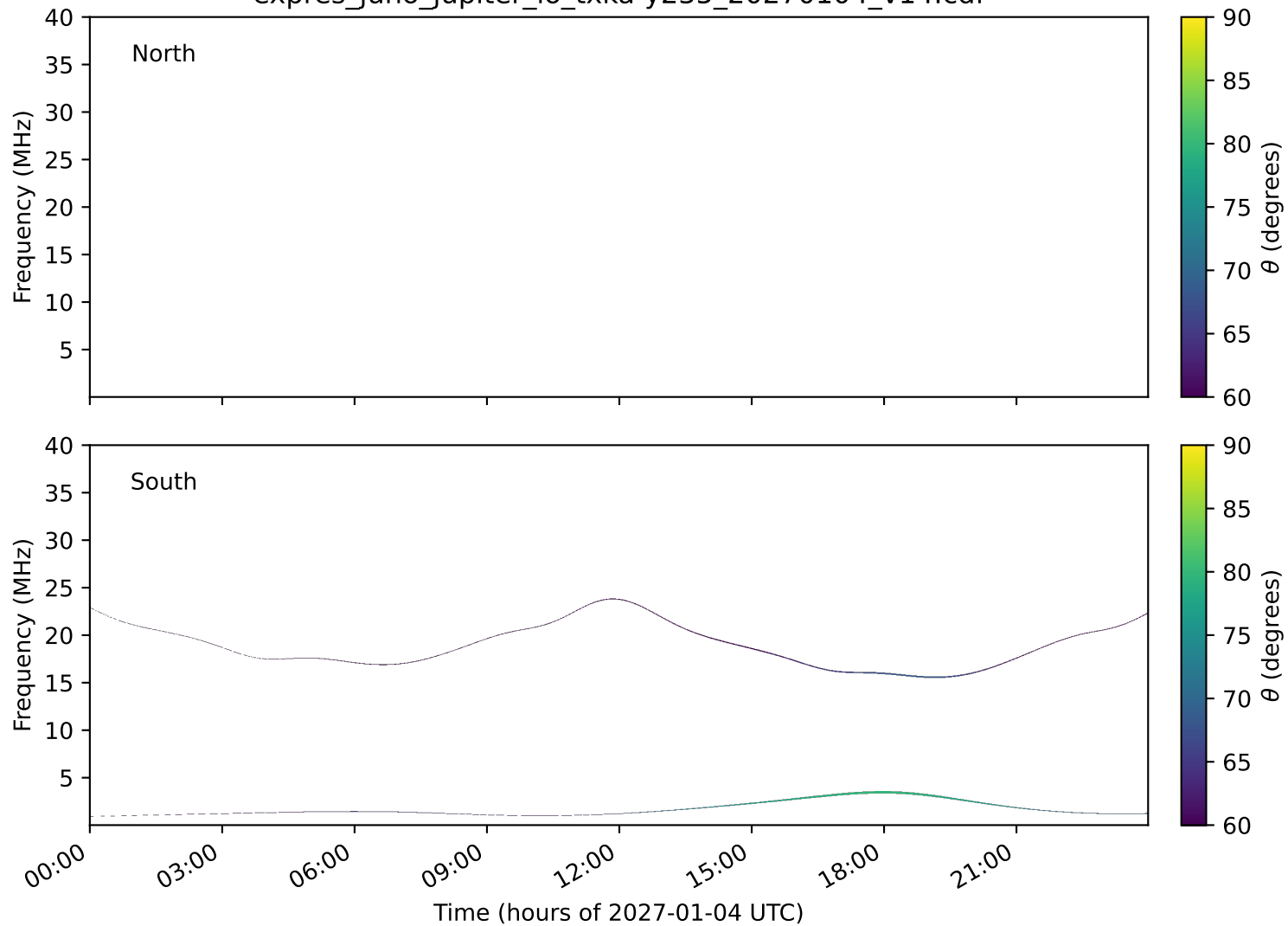
expres_juno_jupiter_io_txka-y235_20270104_v14.cdf
