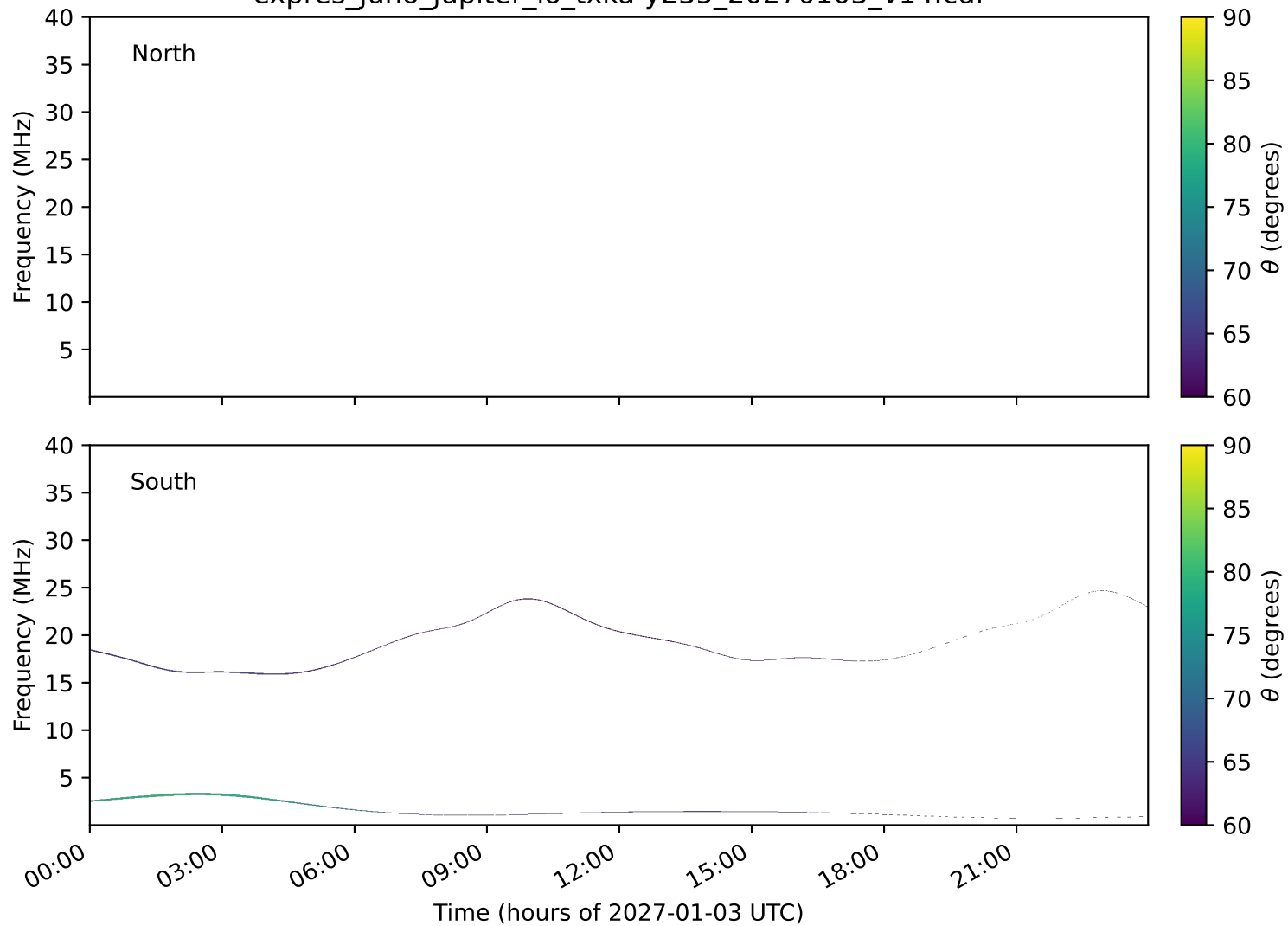
expres_juno_jupiter_io_txka-y235_20270103_v14.cdf
