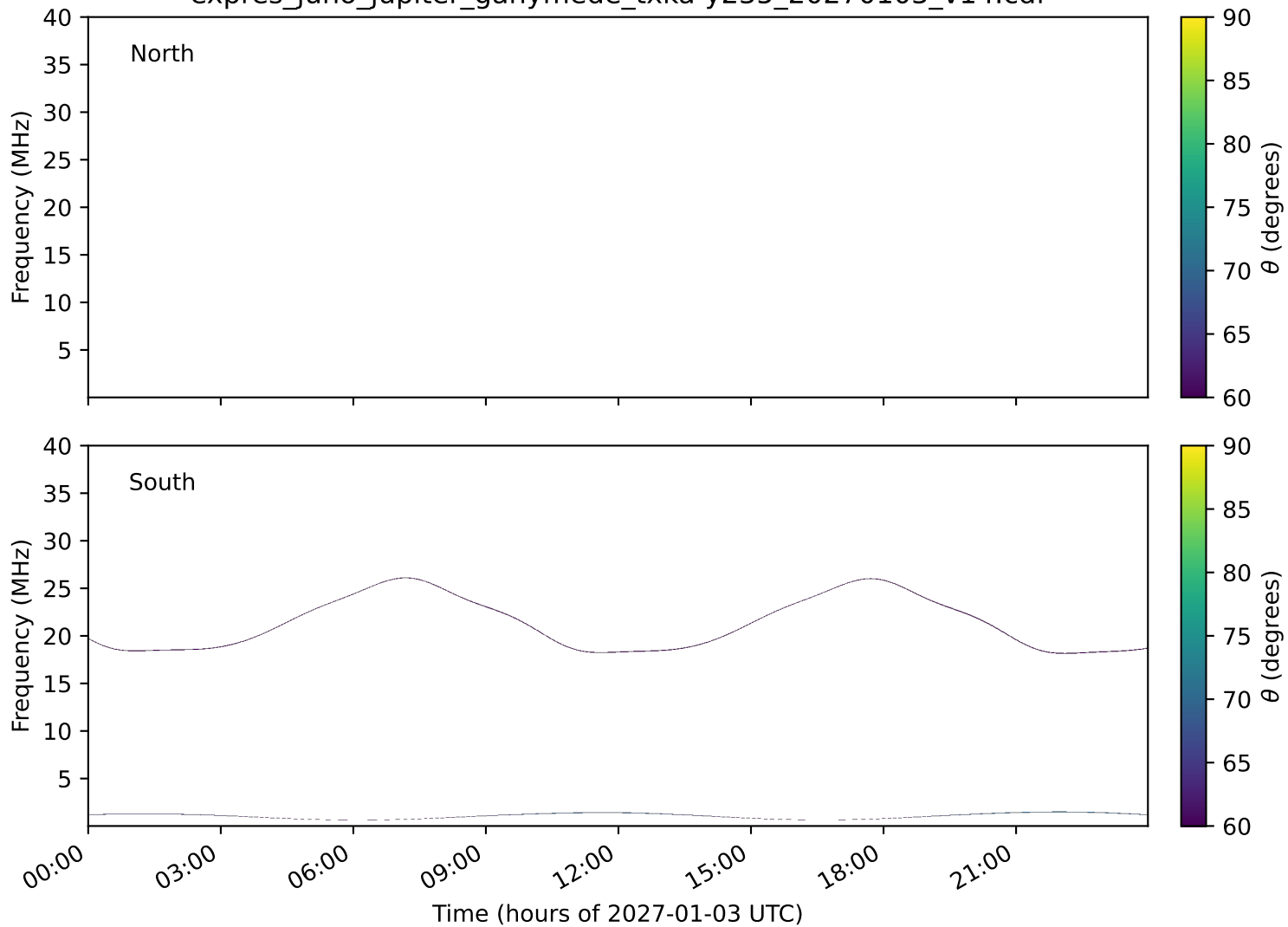
expres_juno_jupiter_ganymede_txka-y235_20270103_v14.cdf
