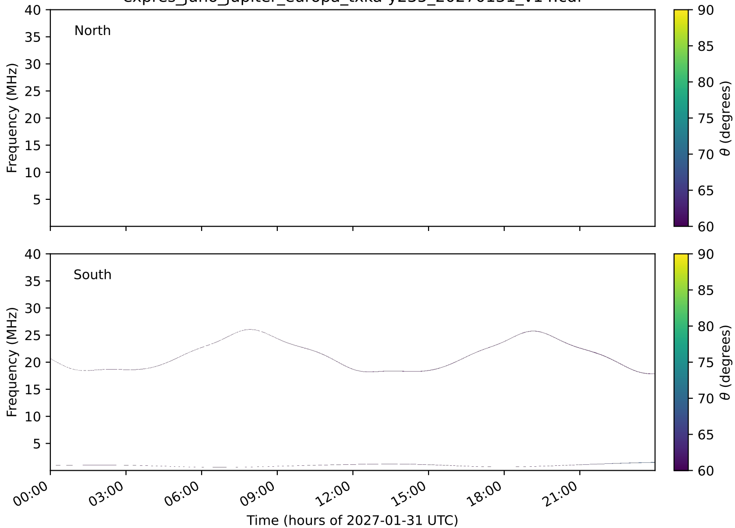
expres_juno_jupiter_europa_txka-y235_20270131_v14.cdf
