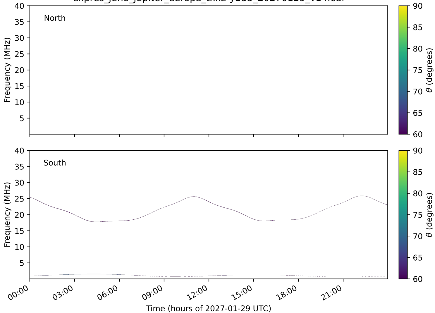
expres_juno_jupiter_europa_txka-y235_20270129_v14.cdf
