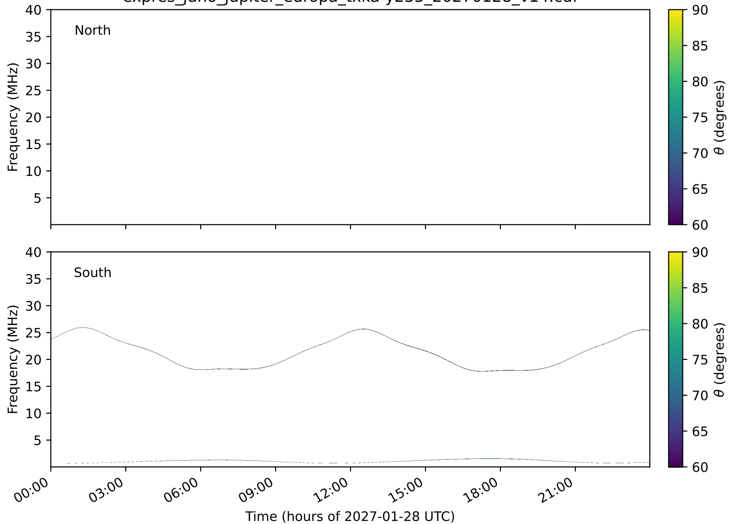
expres_juno_jupiter_europa_txka-y235_20270128_v14.cdf
