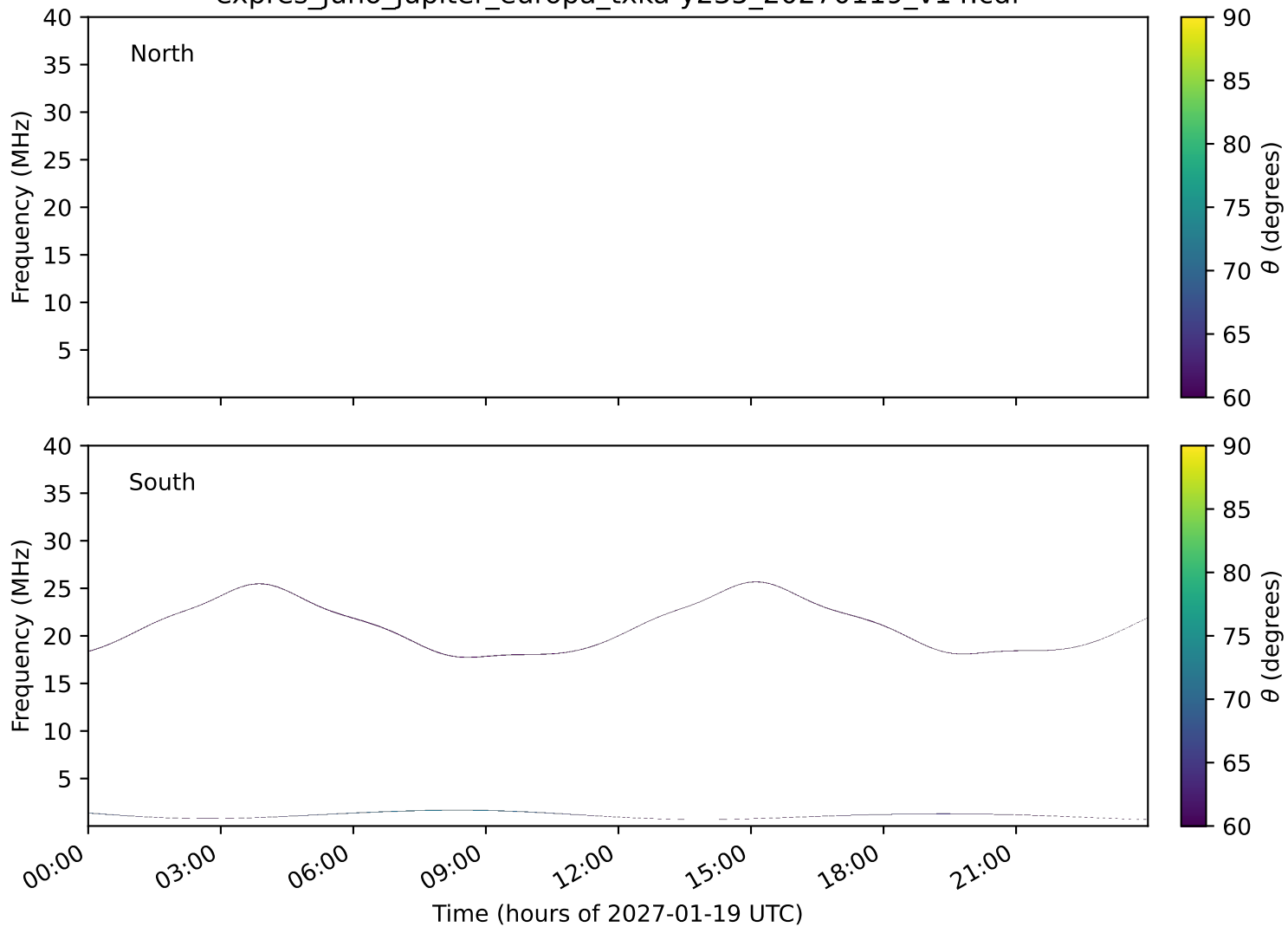
expres_juno_jupiter_europa_txka-y235_20270119_v14.cdf
